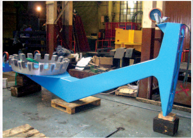
Customer: Royal Observatory Project: Telescope Bracket Use: Bracket for high powered telescope
