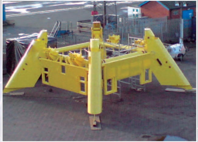
Customer: Vetco Gray Norway Project: Over Trawlable Structure Use: Oil and gas extraction from the seabed
