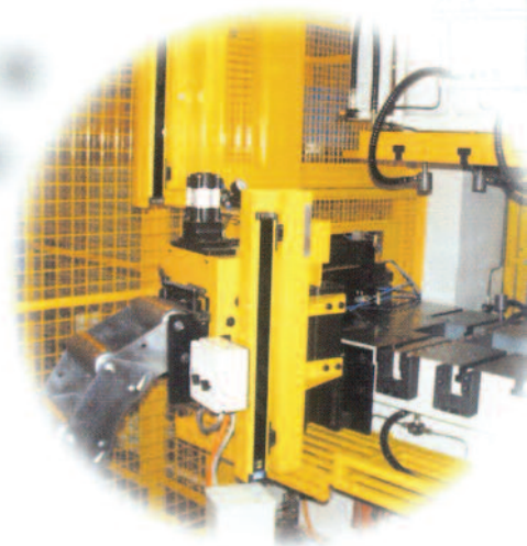
RF60 - Roll Feed on Swivel Mount
