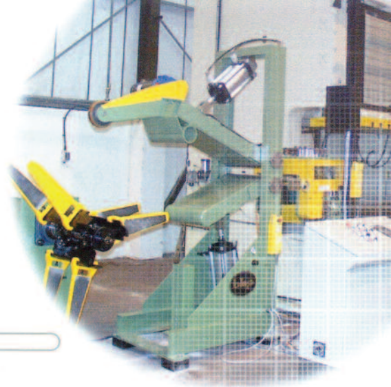
2000kgs x 450mm Feeder Leveller Line
