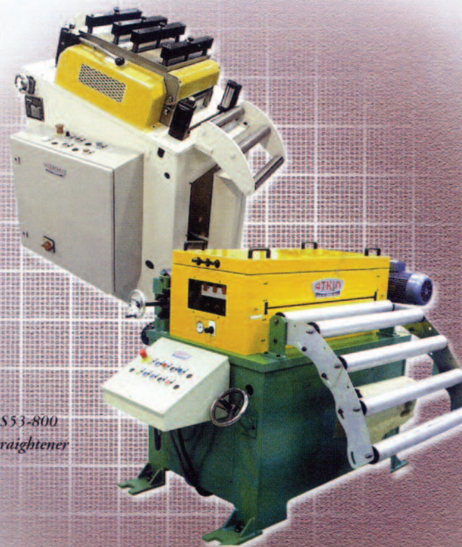
MS59-300 Inclined Head Straightener
